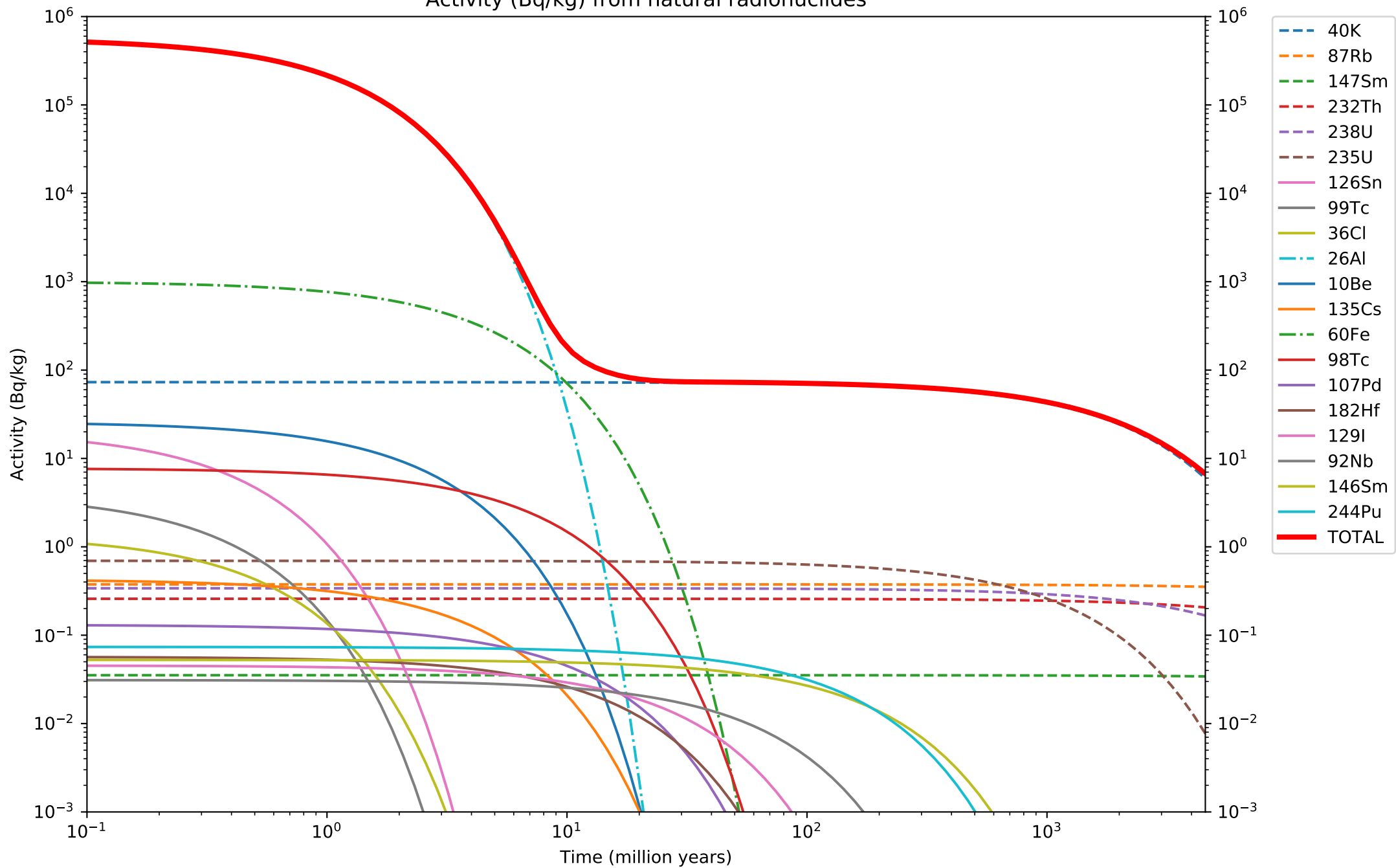
Activity (Bq/kg) from natural radionuclides
