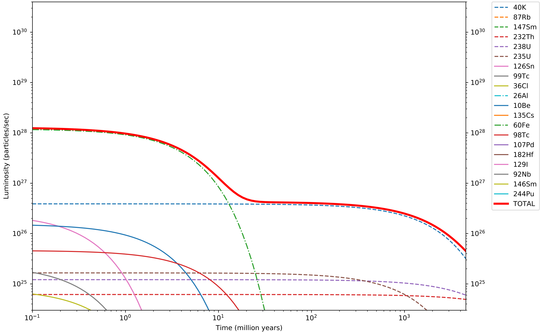
Antineutrino luminosity (particles/sec) from natural radionuclides (antineutrinos only)
