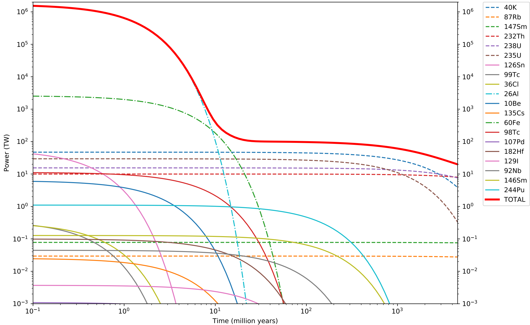
Radiogenic power (TW) from natural radionuclides
