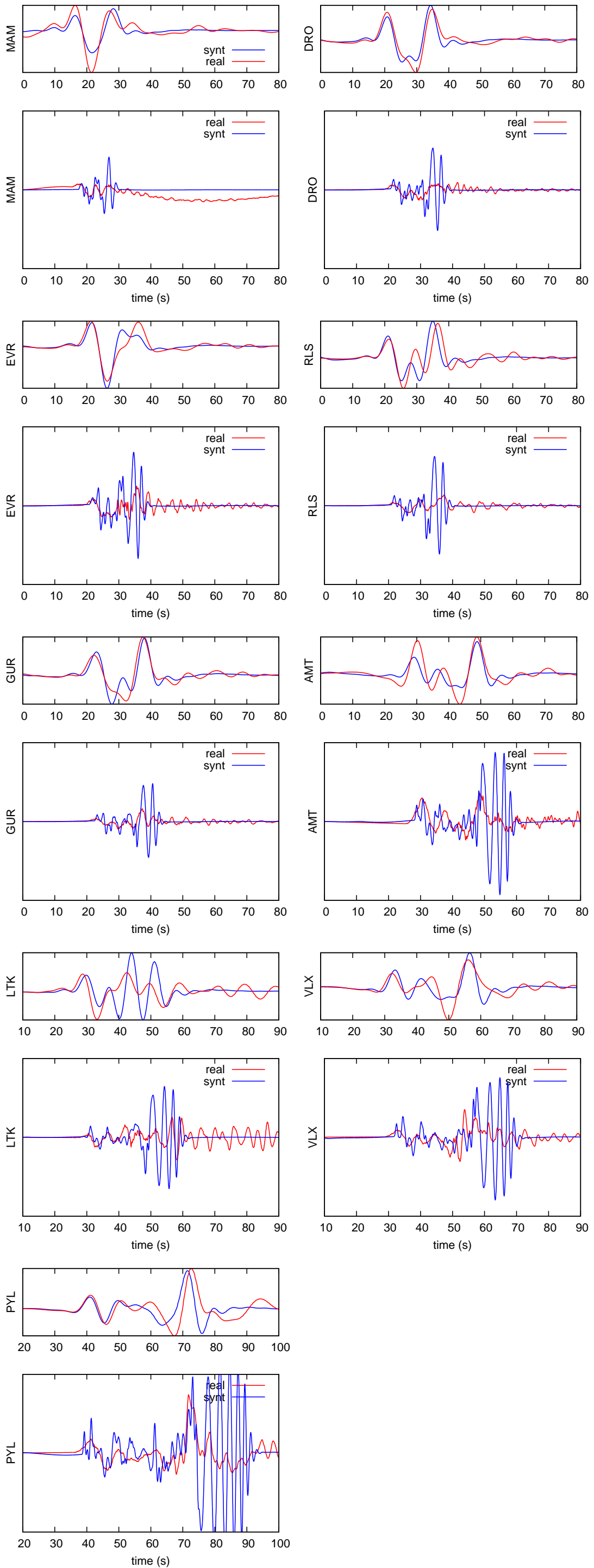
Figure S1: Comparison of the real records (red) and synthetic seismograms (blue) calculated in the best-fitting model. Vertical components at all inverted stations are displayed. Upper panel at each station shows velocity records low-pass filtered up to 0.3 Hz, as used in the waveform inversion. In the lower panels there are displacement records displayed up to 10 Hz to make the PL-wave better visible in context of other waves. The moment-rate function is a 1-s triangle.
